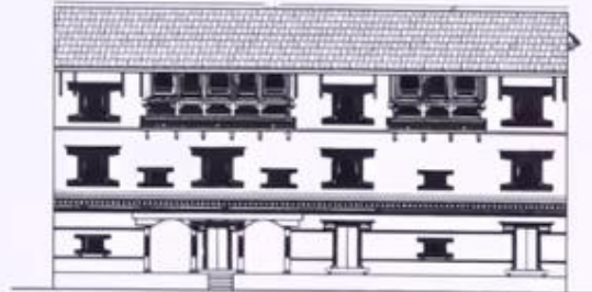
EAST ELEVATION (INNER COURTYARD)
